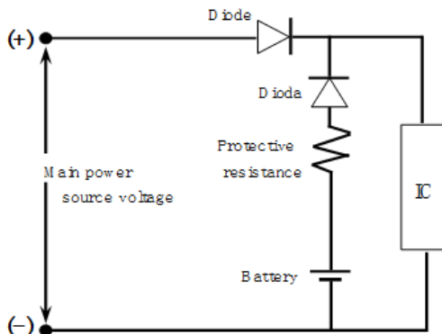
Back-current Prevention Diode and Protection Resistor Used
