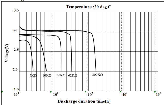
Discharge Characteristics
